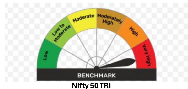
Benchmark
