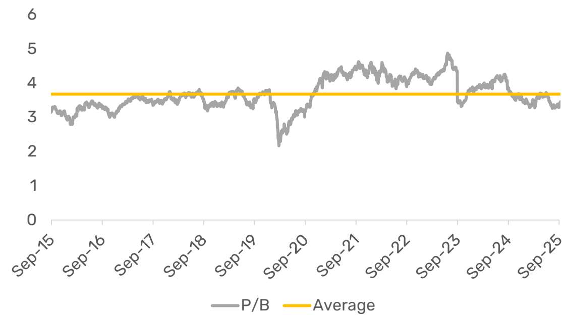
Nifty 50 P/B
